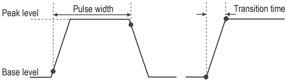
Figure 23. Definition of the pulse parameters and the transition time
