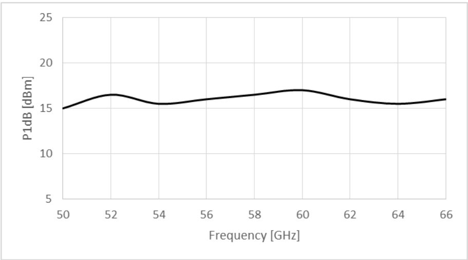
Figure 1: ERZ-HPA-5000-6600-19 P1dB
