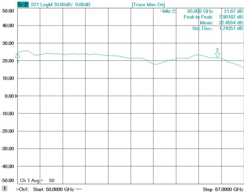
Figure 2: ERZ-HPA-5000-6600-19 Small Signal Gain
