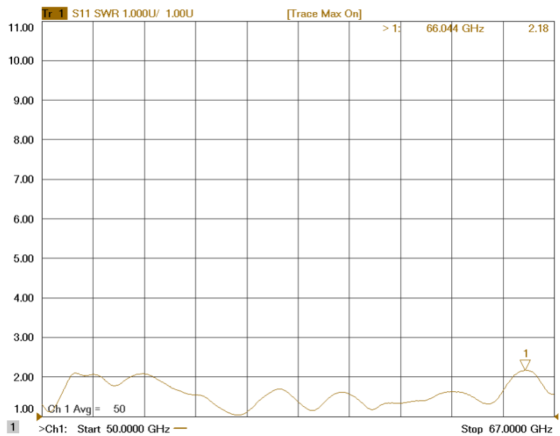
Figure 3: ERZ-HPA-5000-6600-19 Input Matching
