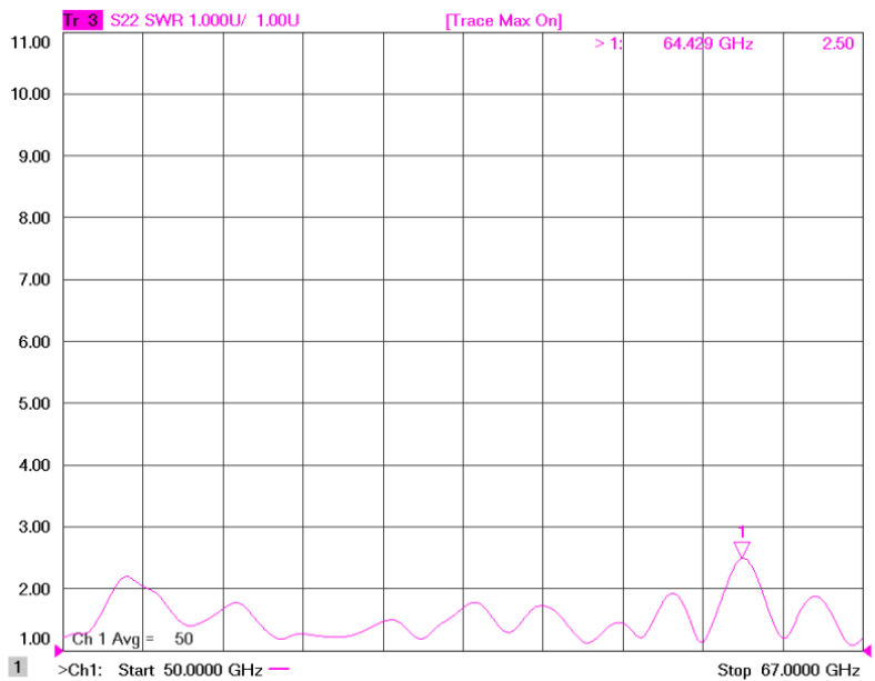
Figure 4: ERZ-HPA-5000-6600-19 Output Matching
