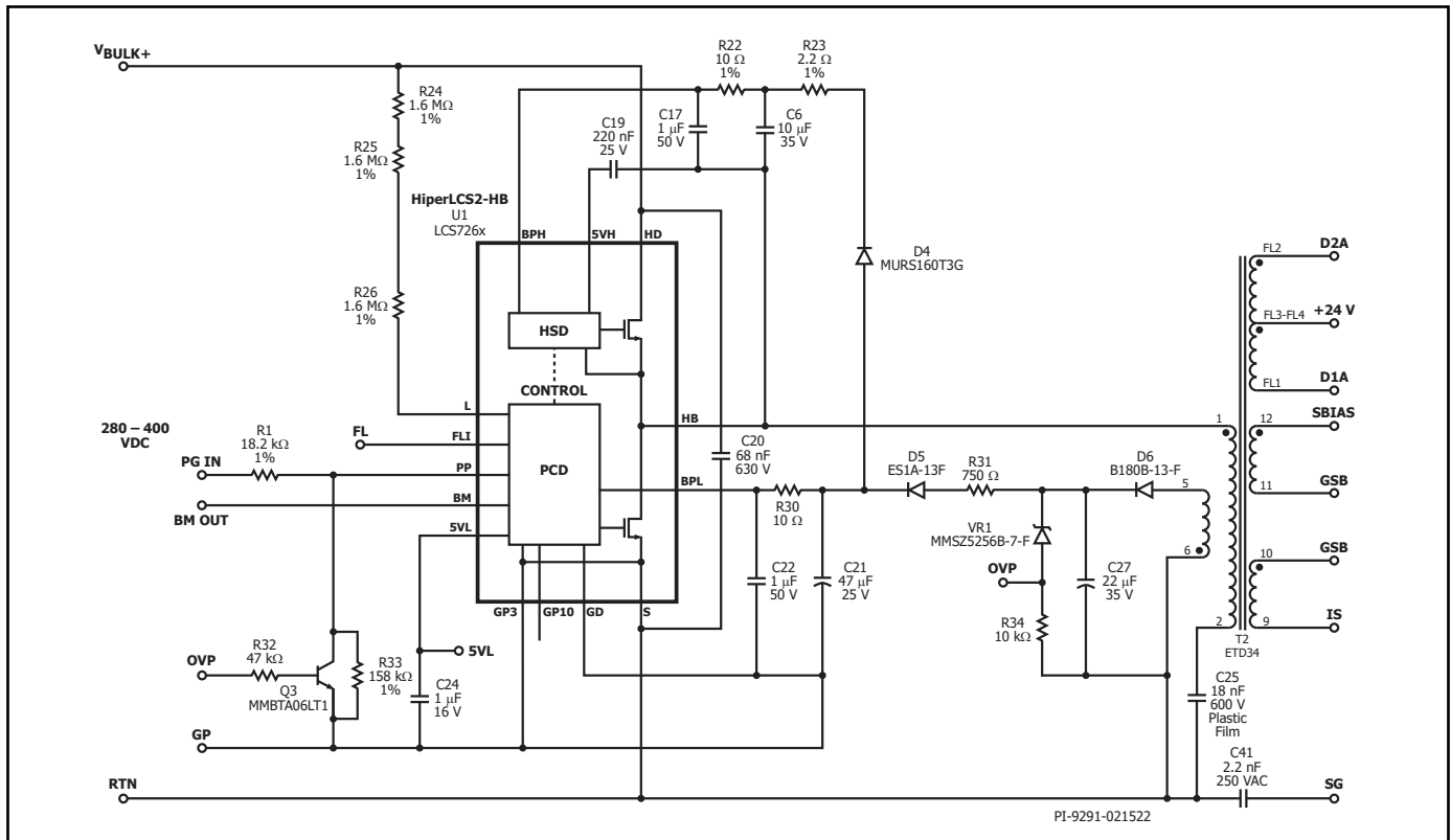
Figure 10. HiperLCS-2 Primary-Side 220 W, 24 V LCS726xC.
