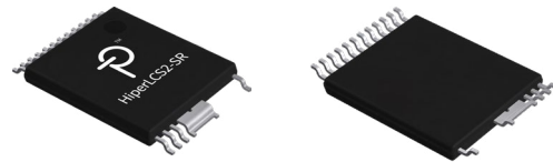
Figure 9. HiperLCS2-SR, Safety Isolation Package. InSOP-24D Top View, InSOP-24D Bottom View.
