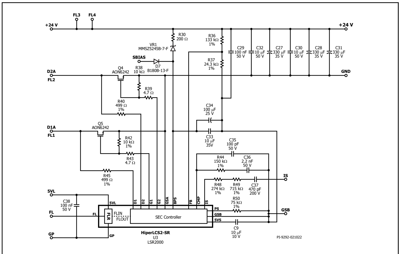
Figure 11. HiperLCS-2 Isolation and Secondary-Side 220 W, 24 V LSR2000C.
