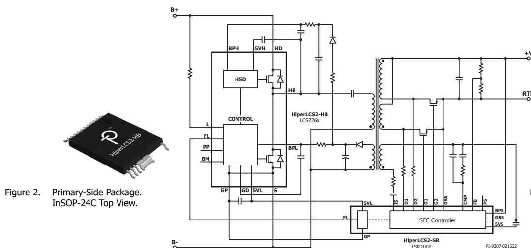
Figure 1. Typical Application Schematic.
