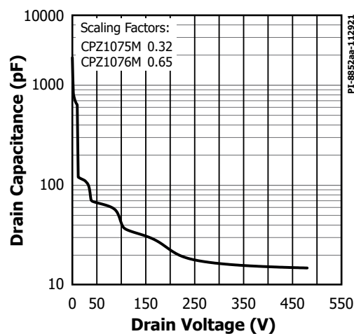
Figure 15. C_{oss} vs. Drain Voltage.
