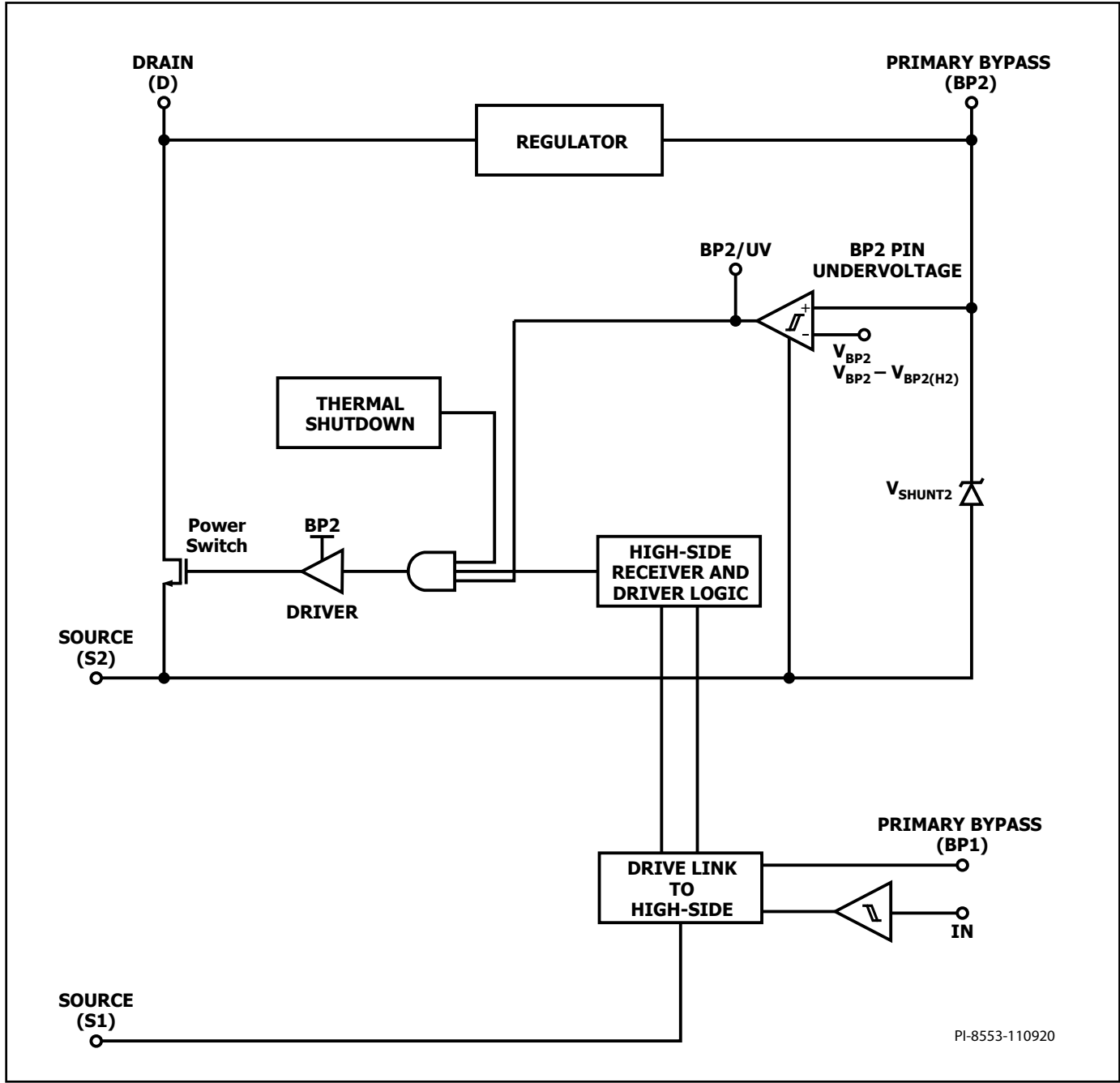
Figure 3. Block Diagram.
