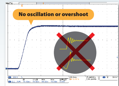
Output voltage waveform with 400 \mu F capacitor connected
