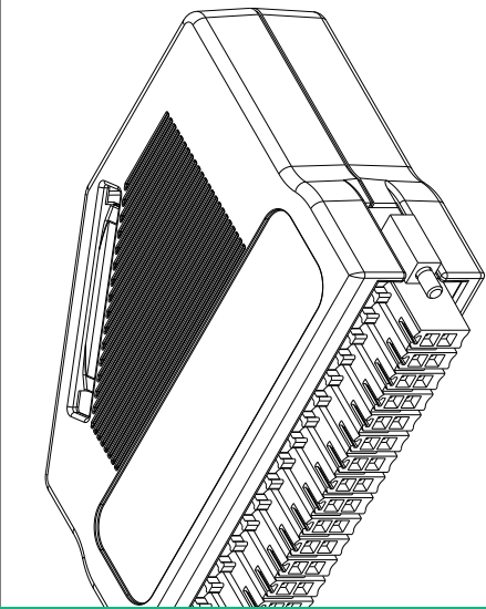
ISOMETRIC VIEW OF 36 PIN CONNECTOR
