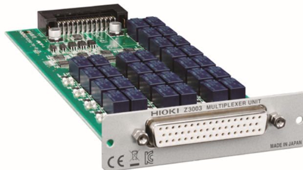
Figure 3: Z3003 multiplexer card
