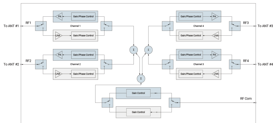
Figure 2. 5G Beamformer System Diagram (4 channels)
