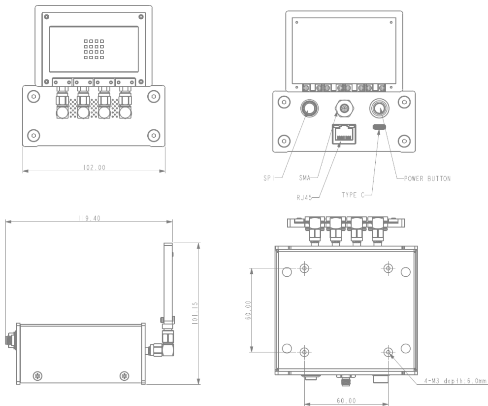
Figure 4. BBox™ Lite Dimension Drawing
