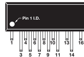
Figure 3. Pin Numbering and Designation.
