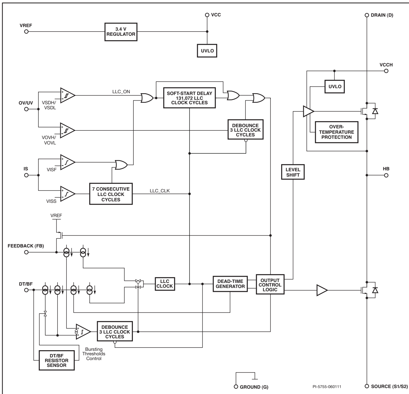
Figure 2. Block Diagram.
