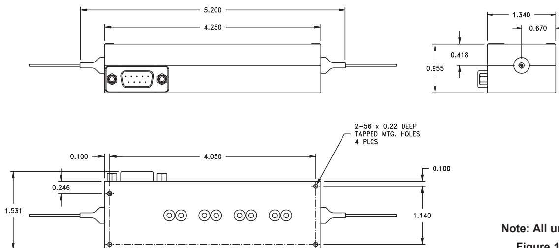
Figure 1: EPC Drawing
