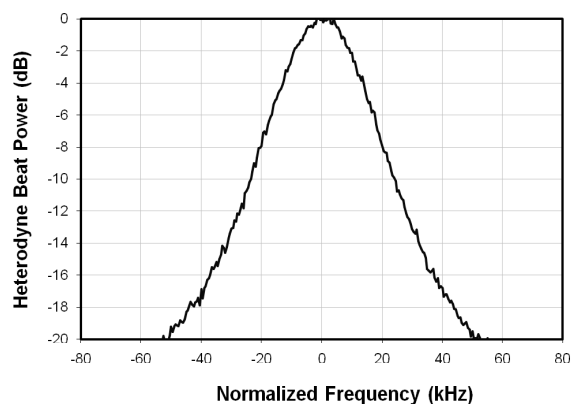
Typical Linewidth Spectrum
