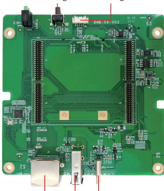
RJ45 Network USB 2.0 DC-IN
