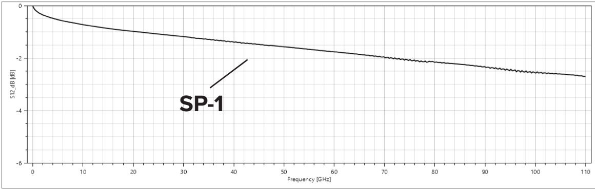
Maury StabilityPlus™ 6" Cable Assembly Typical Insertion Loss
