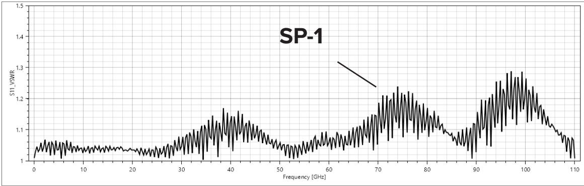
Maury StabilityPlus™ 6" Cable Assembly Typical VSWR
