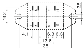
Flange case type
