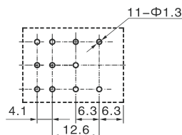
Mounting Holes t (bottom view )
