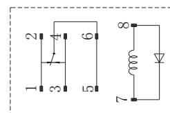
with diode (DC type)
