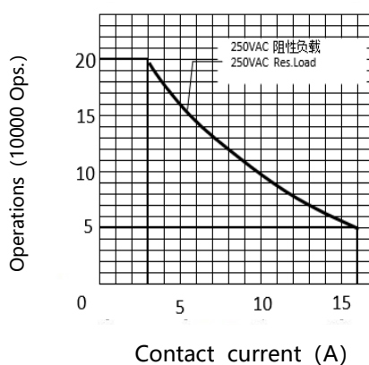
Endurance Curve
