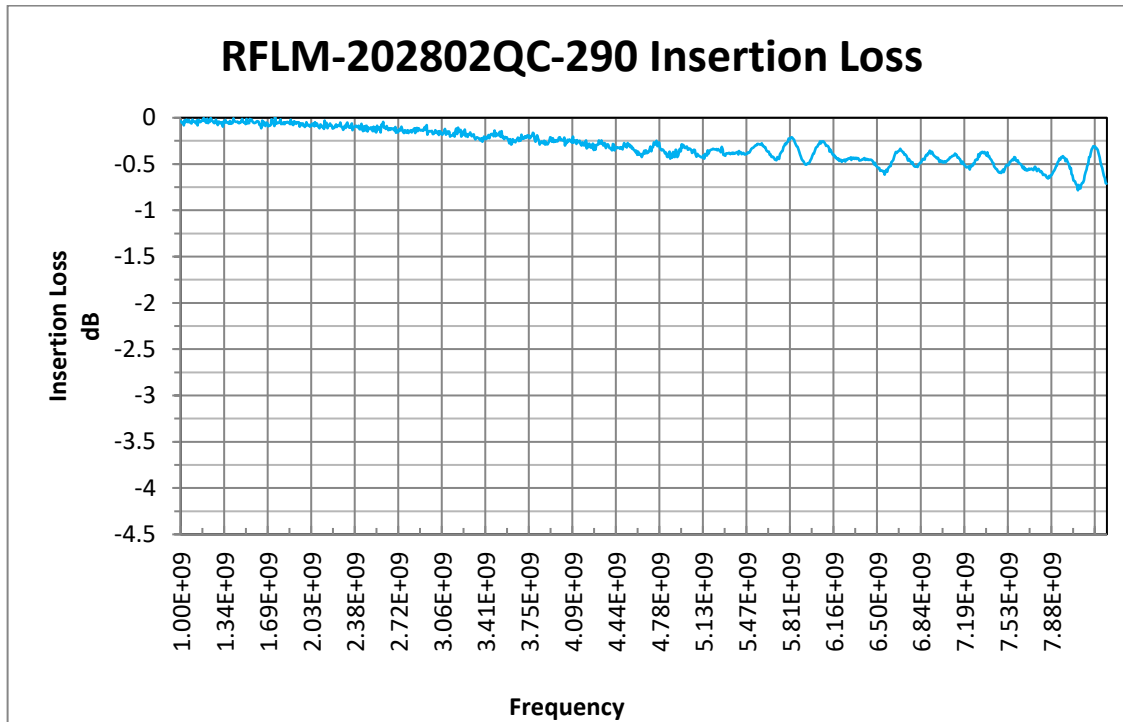
RFLM-202802QC-290 Insertion Loss vs Frequency
