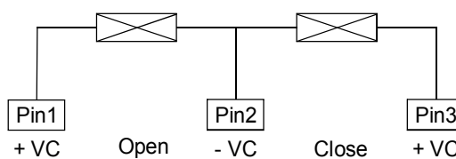
Dual coil
