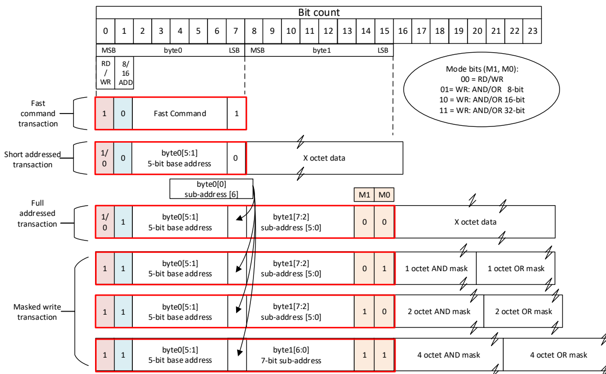
Figure 17: SPI Command Formatting
