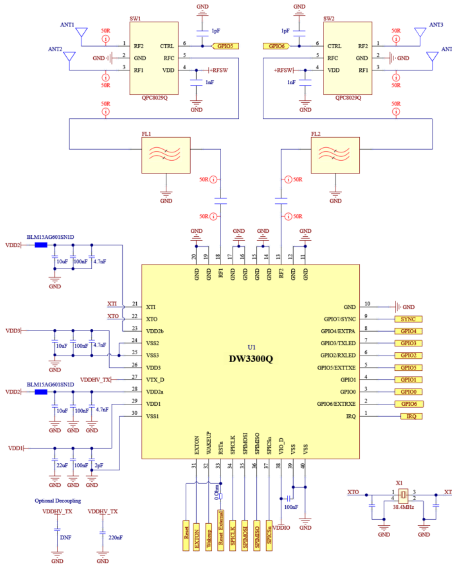
Figure 32: DW3300Q 40 Pin LGA Application Circuit
