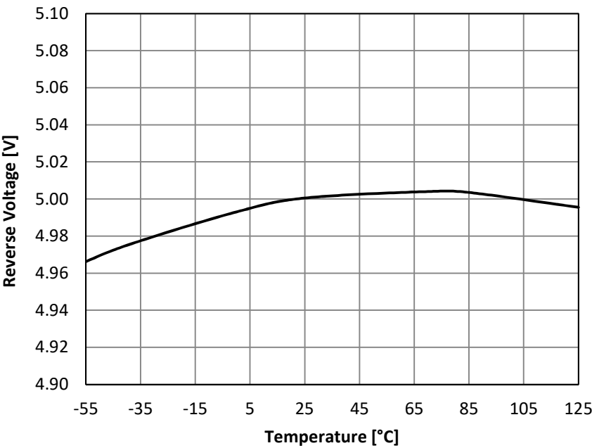
Temperature Drift
