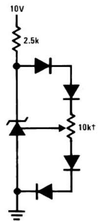
5.0V Reference with Minimum Temperature Coefficient
