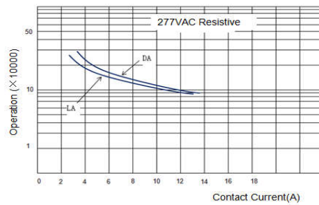
Electrical Life
