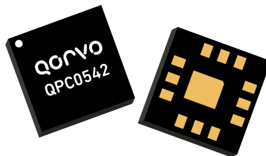
12 Pad 2.25 x 2.25 mm QFN Package
