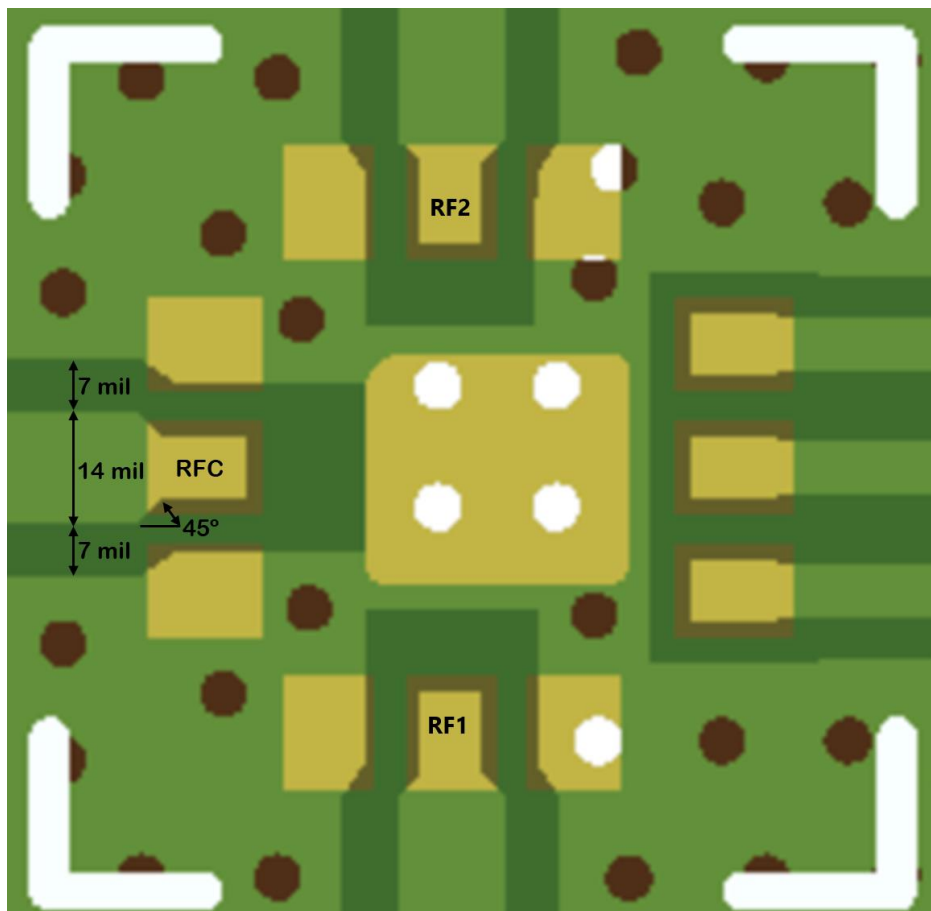
Landing Pattern
