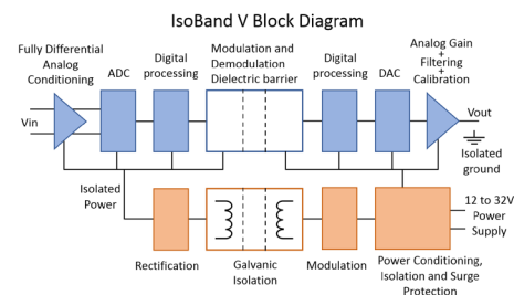
IsoBand V block diagram.
