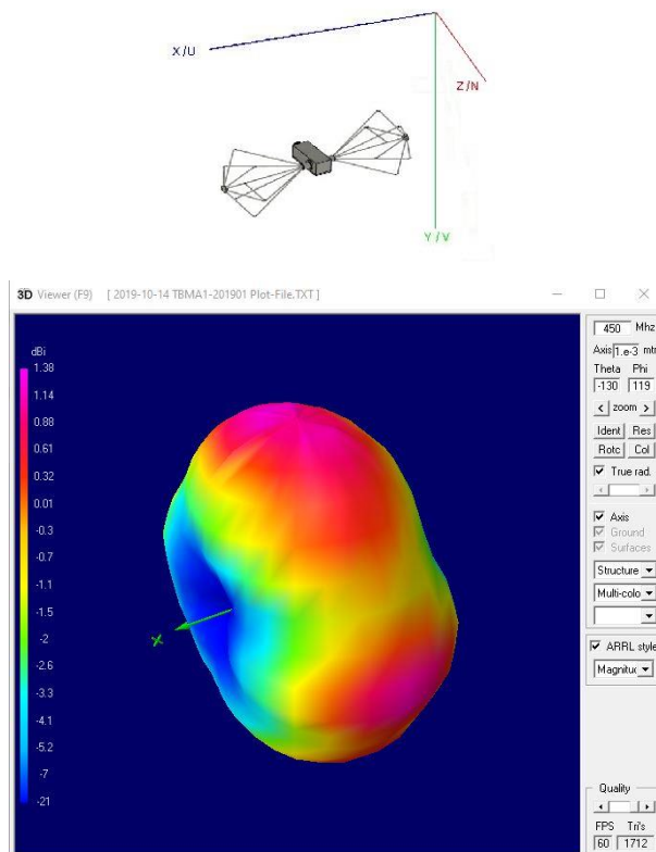
radiation pattern of the TBMA1 at 450 MHz
