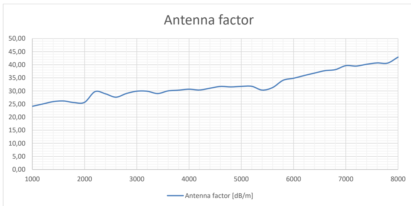
1 GHz...8 GHz, Antenna Factor of TBMA4
