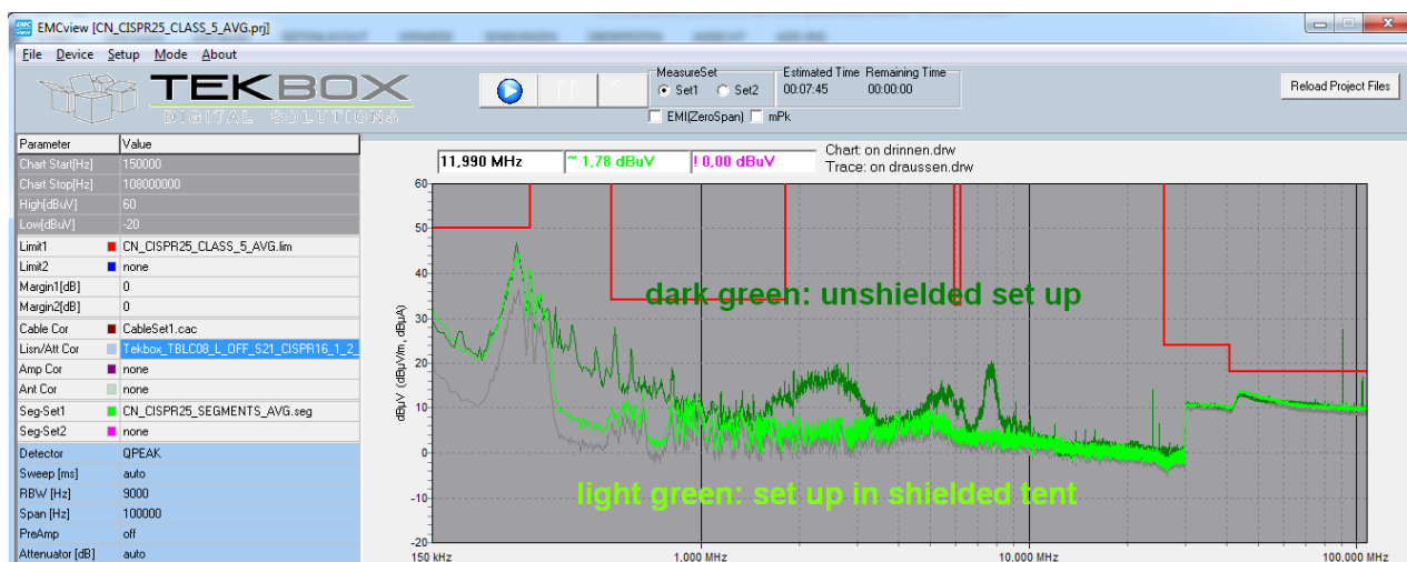
Picture 6: CISPR 25 conducted noise measurement; DUT powered
