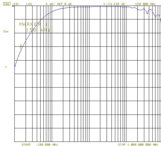
Figure 7 – 100 kHz...1 GHz, insertion loss measured between DUT terminals and BNC connector; source terminals 1 \mu F
