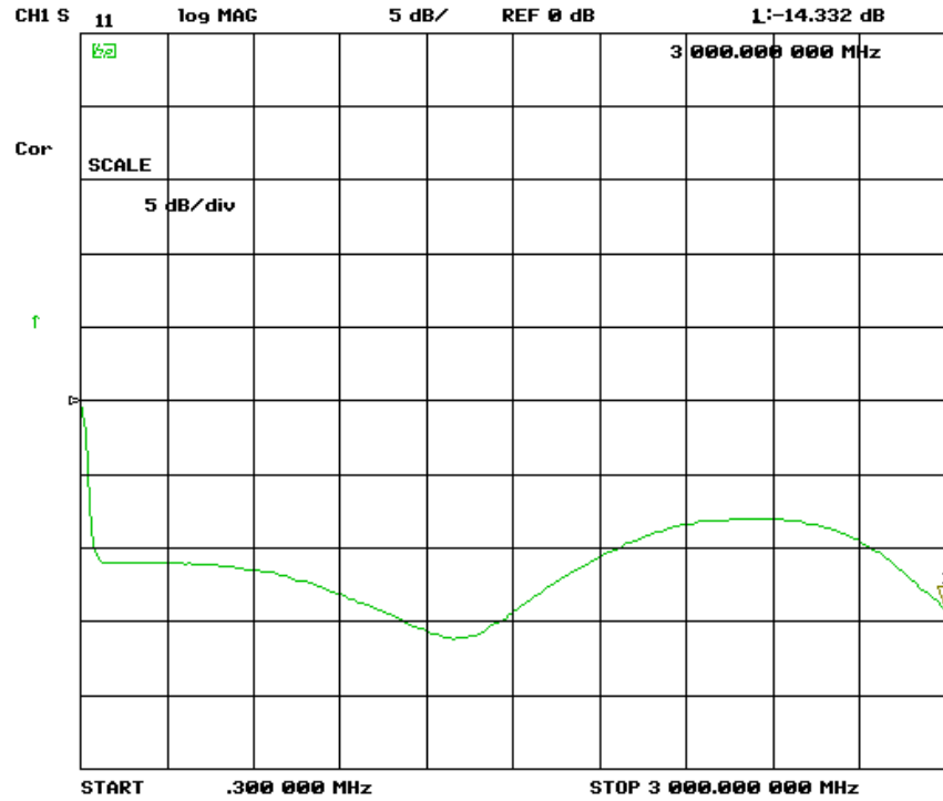
Picture 6 – TBDA1/14dB, input return loss, S_{11} , 300 kHz – 3 GHz, lin.
