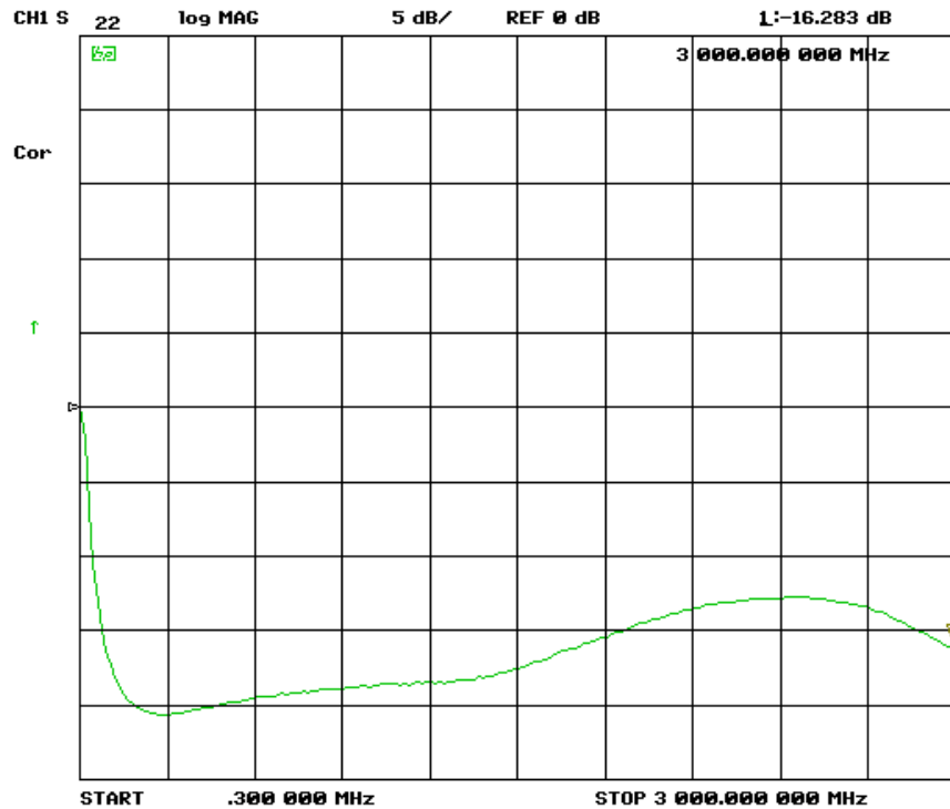
Picture 7 – TBDA1/14dB, output return loss, S_{22} , 300 kHz – 3 GHz, lin.
