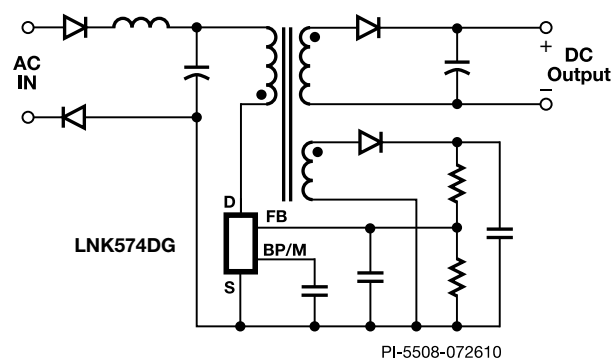
(a) Typical Application Schematic for LNK574DG.
