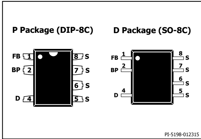
Figure 4. Pin Configuration.
