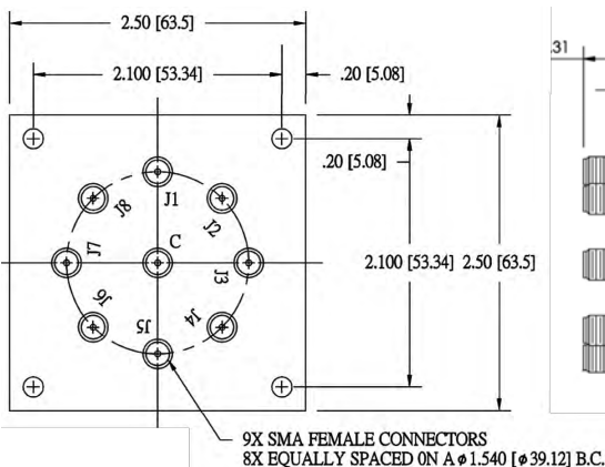
SP8T: 50Ω terminations, 15 pin D-Sub, (Position J1)
