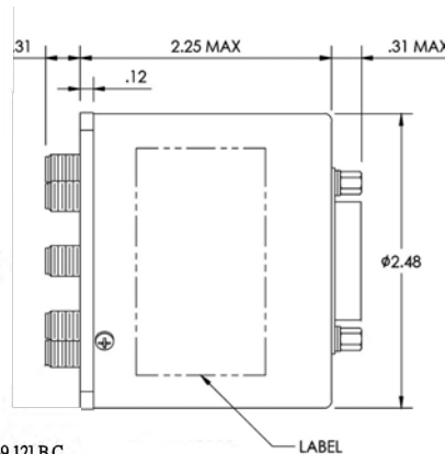
SP8T: 50Ω terminations, 15 pin D-Sub, (Position J1)
