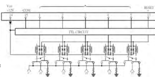
SP5T w/ TTL in position J1
