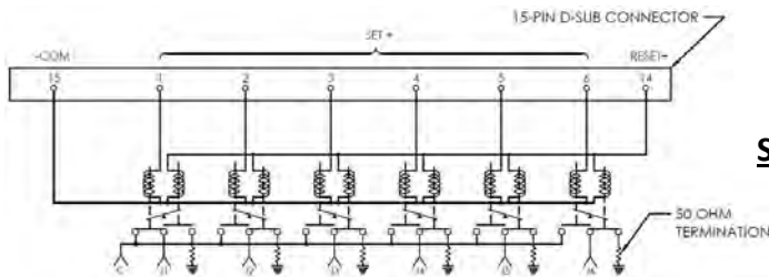
SP6T in position J1
