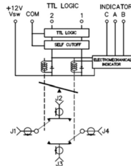
Self Cutoff / TTL + Indicators
