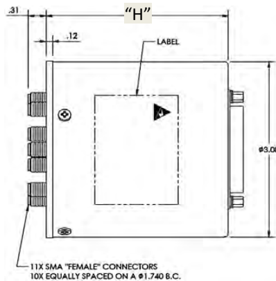
SP10T: 50Ω terminations, 15 pin D-Sub
