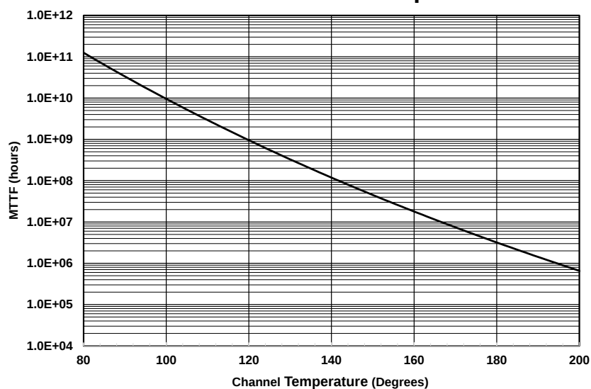
MTTF vs Channel Temperature
