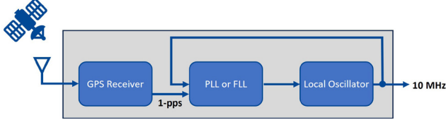
Figure 1: A typical “black box” GPS-receiver (antenna in - reference out). Internal oscillator offset and adjustments are invisible to the user.
