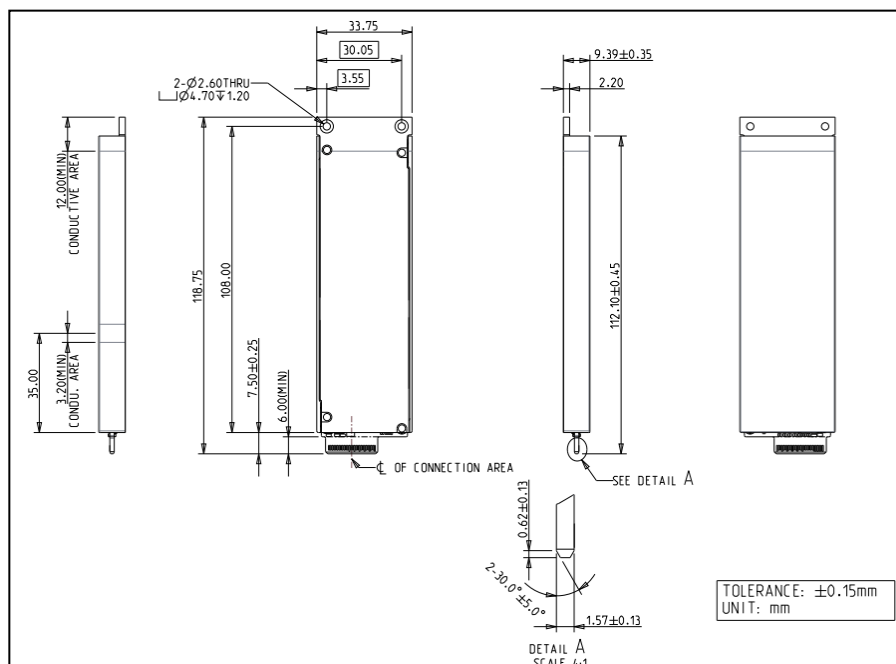
Figure 2: Innodisk E1.S 4TS2-P with 9.5mm enclosure
