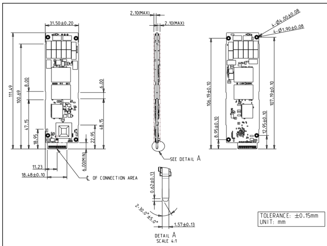
Figure 4: Innodisk E1.S 4TS2-P 5.9mm (400GB-3.2TB)
