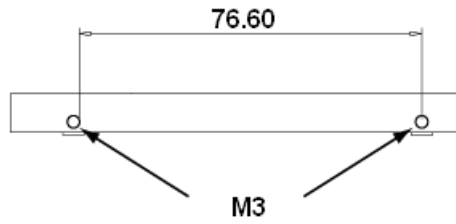
Figure 6: 2.5" SATA SSD 3TS9-P Mechanical Screw Hole
