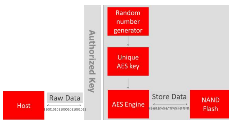
Figure 4: Innodisk 2.5" SATA SSD 3TS9-P AES flow chart
