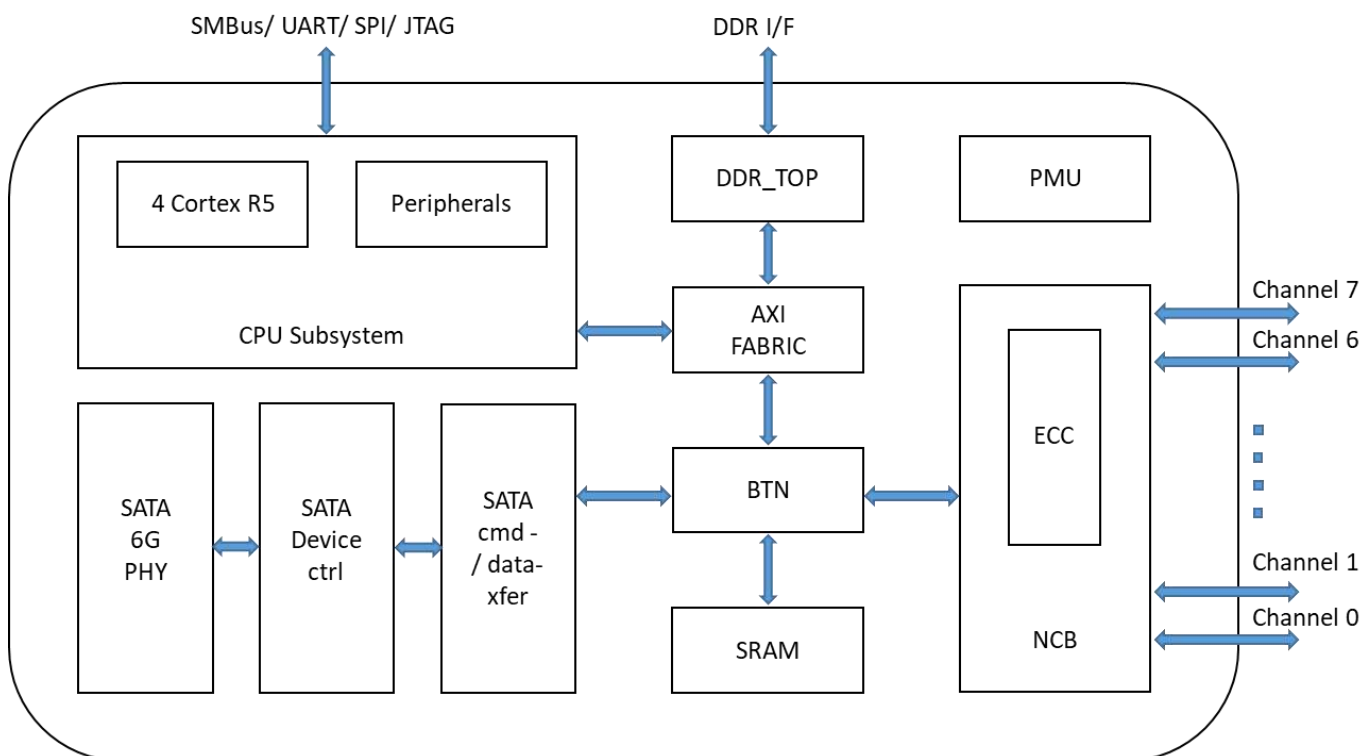
Figure 2: Innodisk 2.5" SATA SSD 3TS9-P Block Diagram
