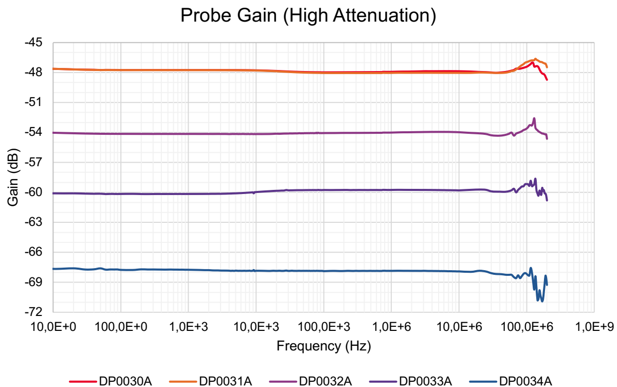
Figure 2. Vout/Vin frequency response of DP003xA probes on high attenuation settings.
