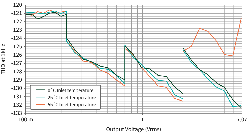
Figure 35. THD of 1 kHz Tone Amplitude Sweep
