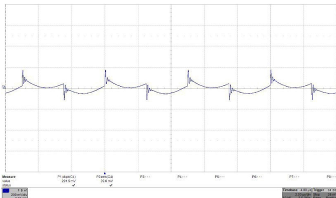
Fig. 26: Output voltage ripple (200mV/div.) at full rated load current into a resistive load at VIN = 24V. C_0 = 470\mu F/70m\Omega . Time: 2μs/div.
