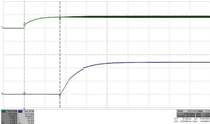
Fig. 8: Turn-on by ON/OFF transient (with VIN applied) at full rated load current (resistive) at VIN = 24V. Top trace (C1): ON/OFF signal (5V/div.). Bottom trace (C4): Output voltage (10 V/div.). Time 5 ms/div.
