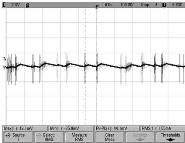
Ripple and Noise @25°C (Vin=110V, Vout=nom., Iout=0, Cloud=0, ScopeBW=20MHz, 100μS/div)
