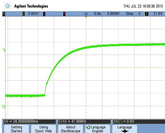
Start-up into a Pre-bias Load@25°C (Vin=57.6V, Prebias V = 4v, Cloud=0μ, 5mS/div)
