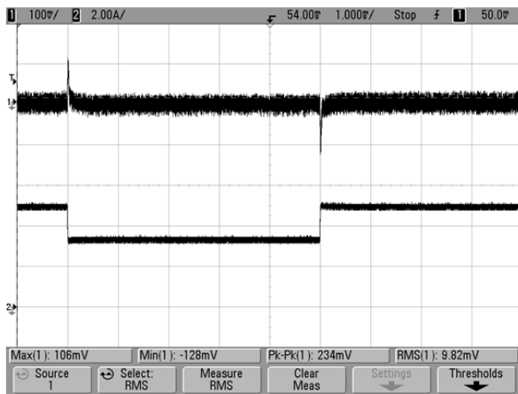
Step Load Transient Response@25°C (Vin=110V, Vout=nom., Iout=50-75-50% of fullload, Cloud=0μF, ScopeBW =20MHz, 54mS/div)
