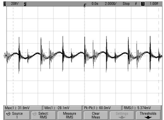
Ripple and Noise @25°C (Vin = 110V, Vout = nom., Iout= 6.3A, Cloud = 0, ScopeBW = 20MHz, 2μS/div)
