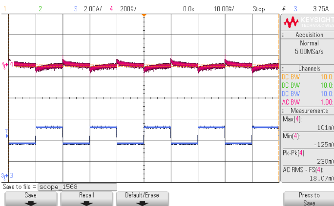
Output voltage response to step-change in load current (50%-75%-50% of full load; di/dt = 0.1A/μs)
