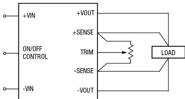
Figure 8. Trim Connections Using a Trimpot
