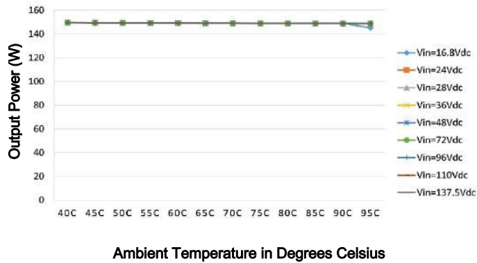
Temperature Derating
