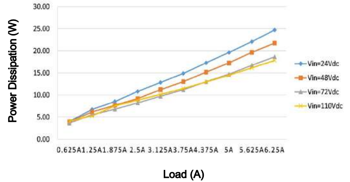
Power Dissipation vs Load
