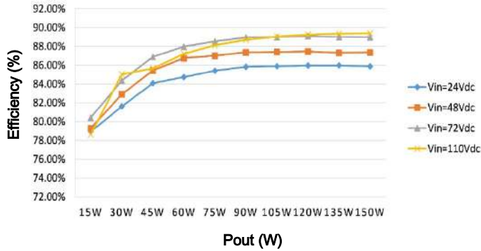
Efficiency vs Pout
