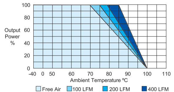
Derating Curve
