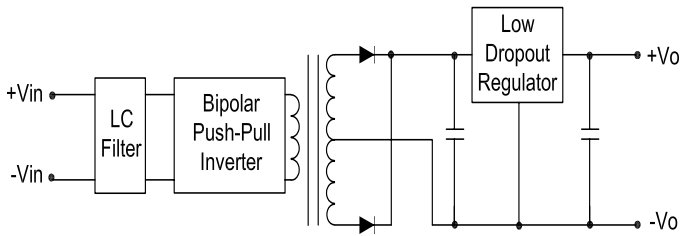
Single Output Block Diagram
