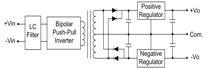
Dual Output Block Diagram
