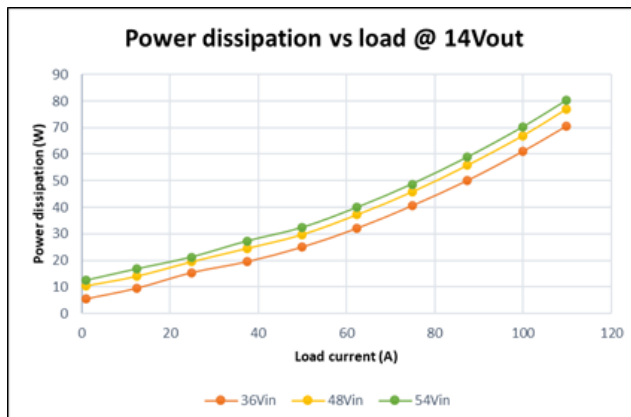
Figure 4: 48S12.1K5BCA Power Dissipation – Buck Mode, V_o=14V
