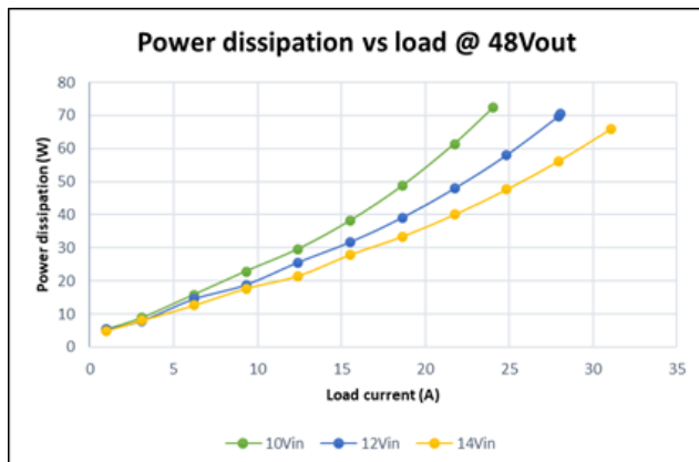
Figure 6: 48S12.215BCE-A Power Dissipation – Boost Mode
