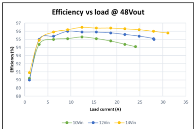
Figure 5: 48S12.1K5BCA Efficiency Curve – Boost Mode, V_o=48V
