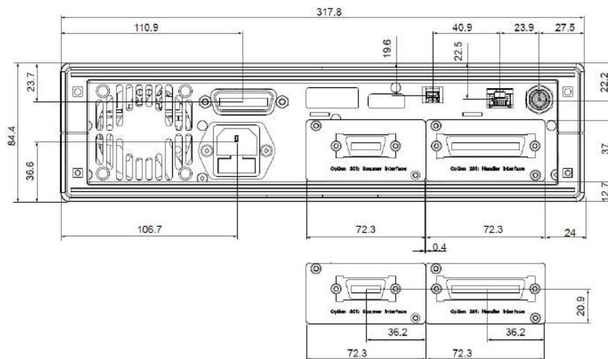
Figure 5. Dimensions (rear view, with handle and bumper, in millimeters, nominal)
