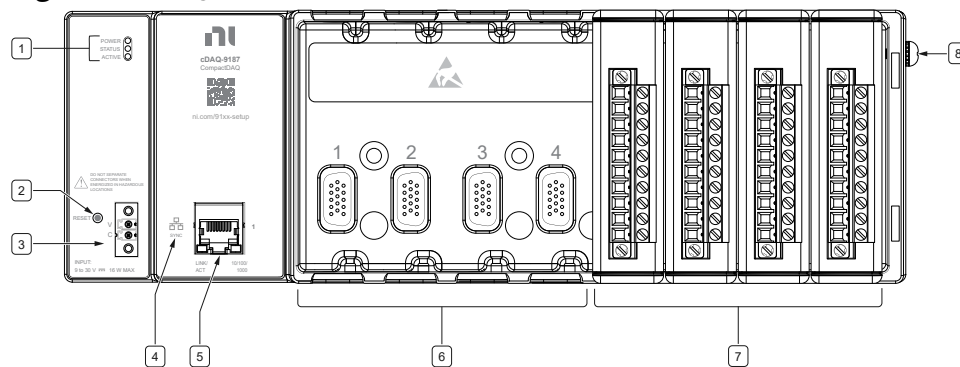
Figure 1. cDAQ-9187 Front Panel
