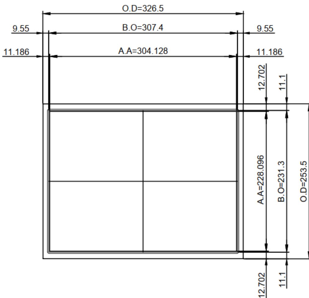
Back view
