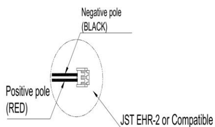
Connector View
