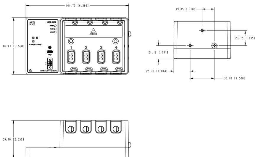
Figure 1. cDAQ-9173 Dimensions
